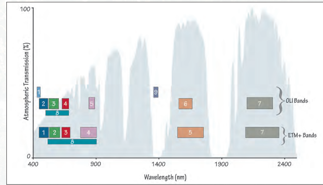
This graph compares the portions of the electromagnetic spectrum that Landsat 7's Enhanced Thematic Mapper-Plus (ETM+) observed (lower row) to the parts of the spectrum that LDCM's OLI will observe (upper row). Note that OLI will detect two new spectral bands labeled 1 and 9 in the upper row.
